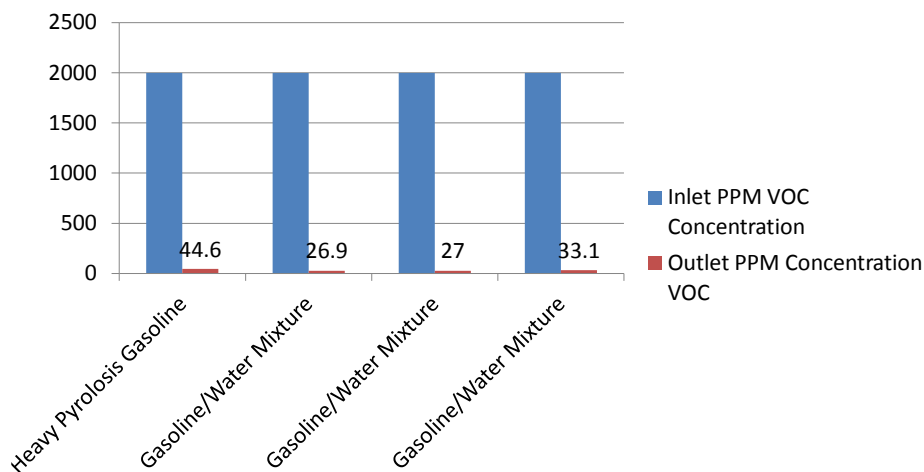
Single Liquid Scrubber with Vapor Scrub EZ Continuous Vacuum Load Method 150-250 CFM Inlet Flow Rate
