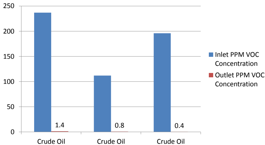
Single Liquid Scrubber with Vapor Scrub EZ Continuous Vacuum Load Method 150-250 CFM Inlet Flow Rate
